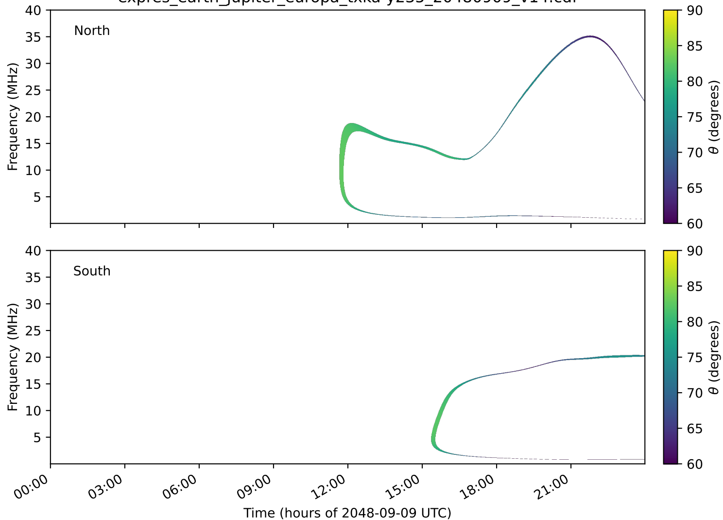
expres_earth_jupiter_europa_txka-y235_20480909_v14.cdf
