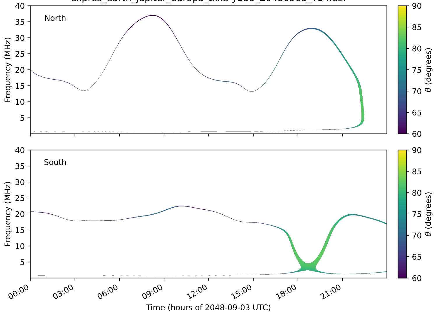
expres_earth_jupiter_europa_txka-y235_20480903_v14.cdf
