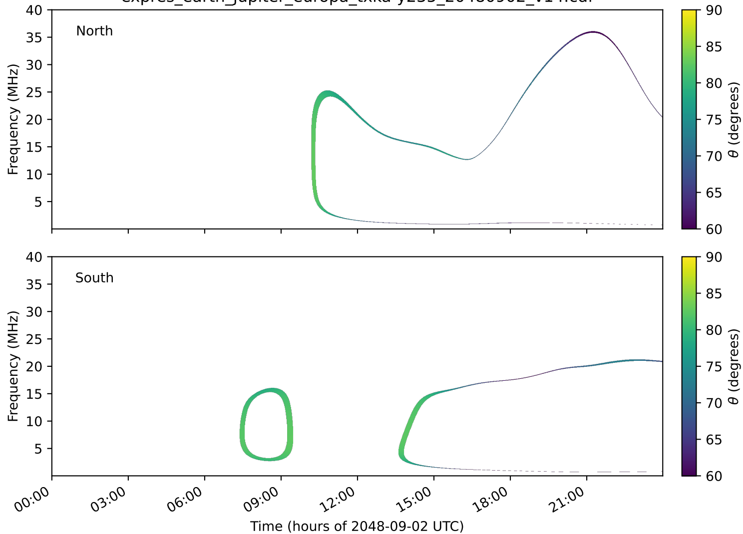
expres_earth_jupiter_europa_txka-y235_20480902_v14.cdf
