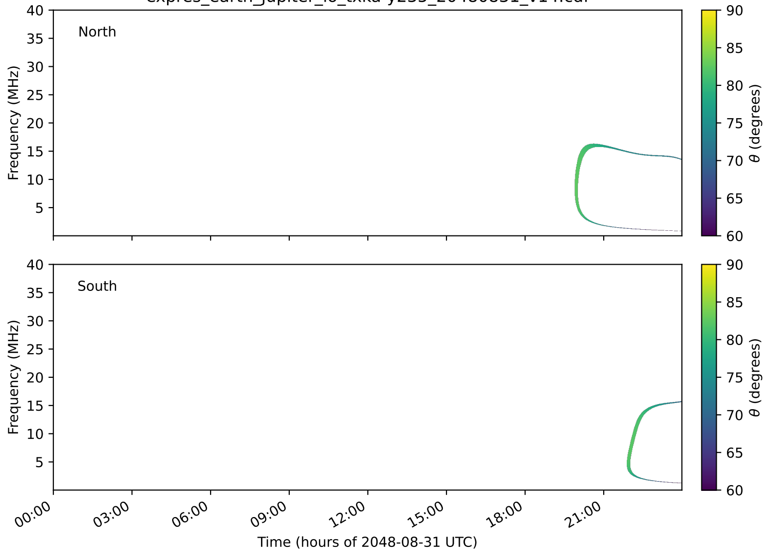
expres_earth_jupiter_io_txka-y235_20480831_v14.cdf
