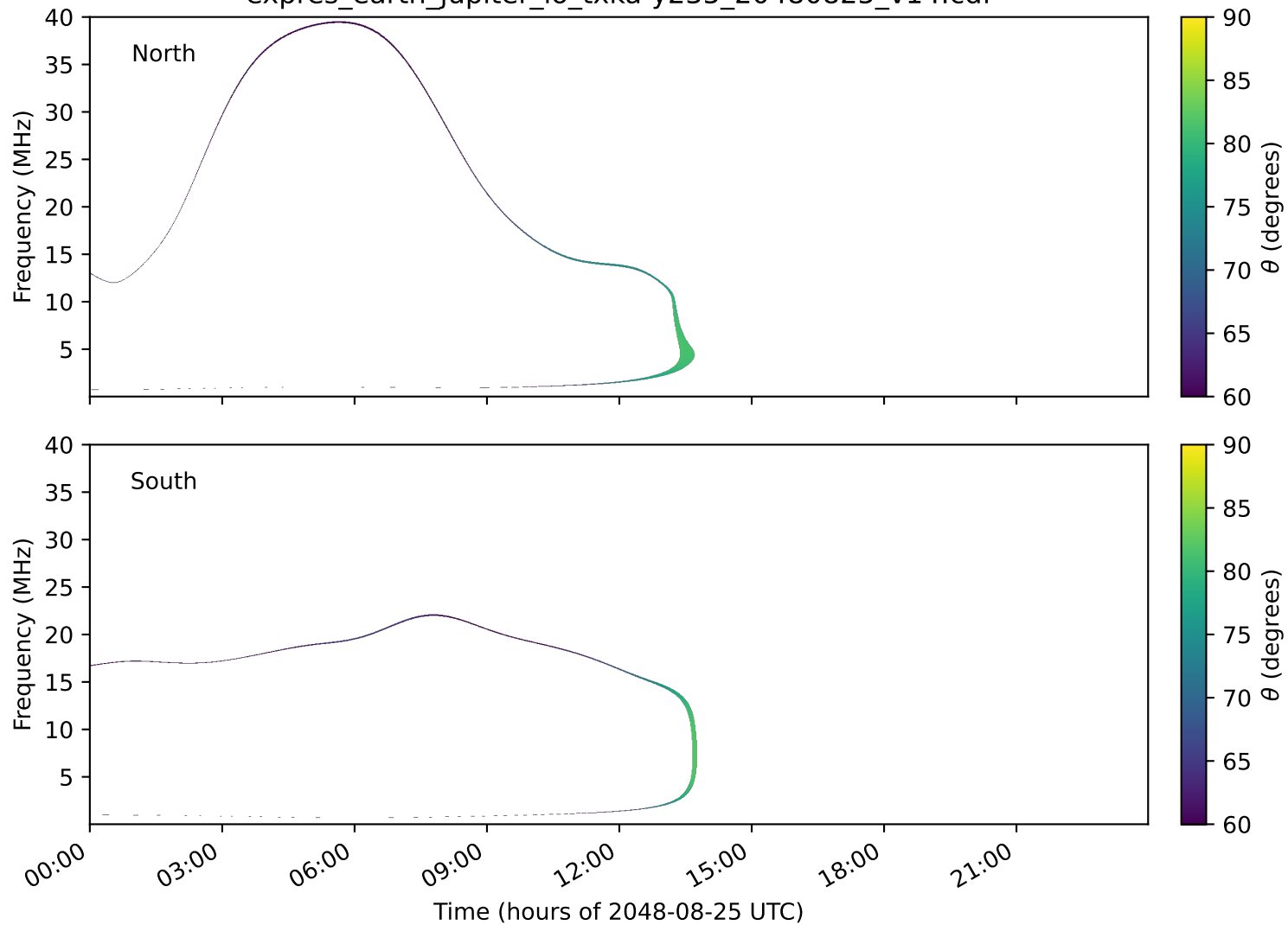
expres_earth_jupiter_io_txka-y235_20480825_v14.cdf
