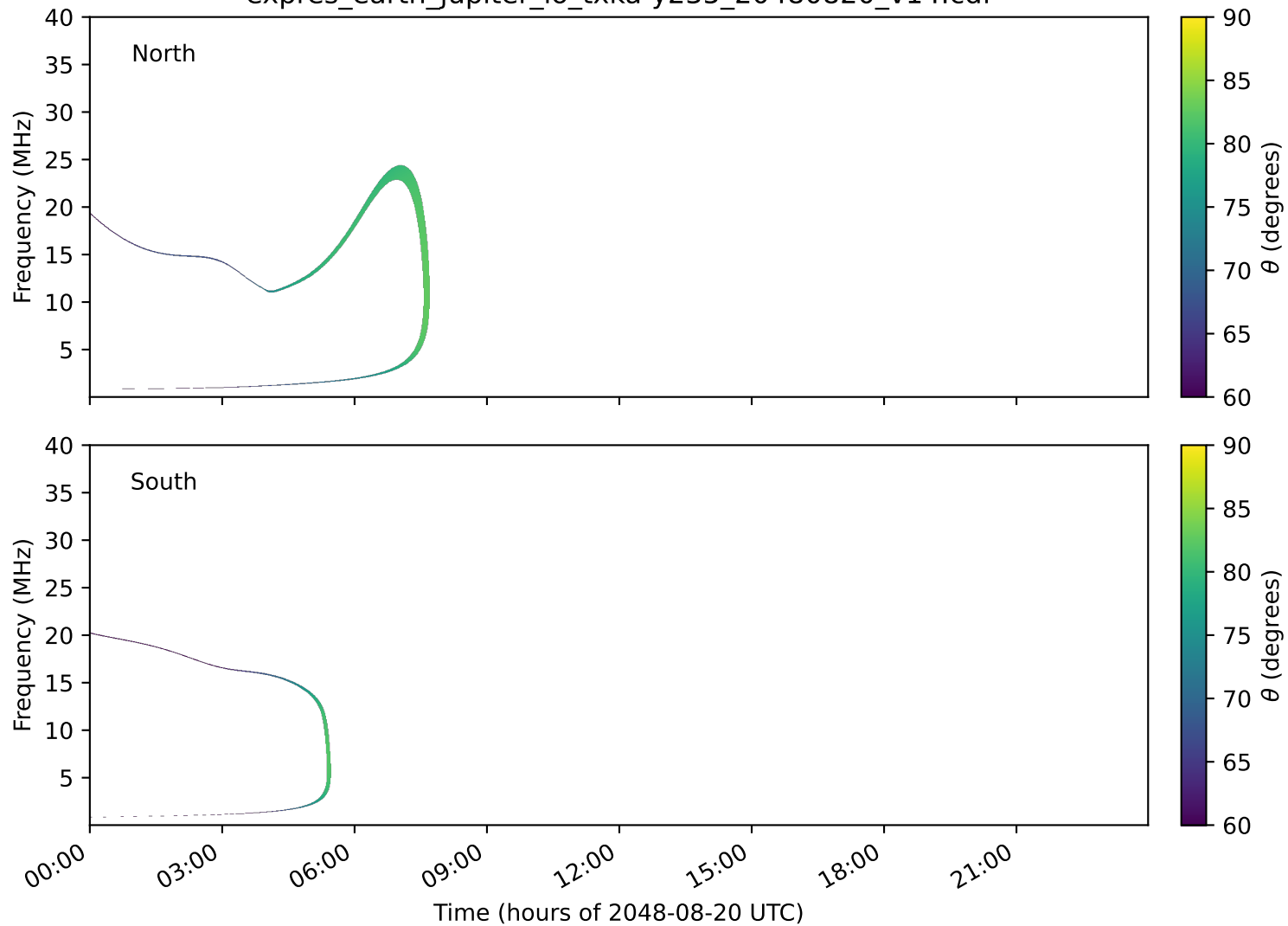
expres_earth_jupiter_io_txka-y235_20480820_v14.cdf
