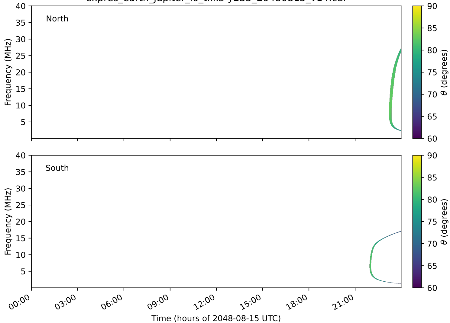
expres_earth_jupiter_io_txka-y235_20480815_v14.cdf
