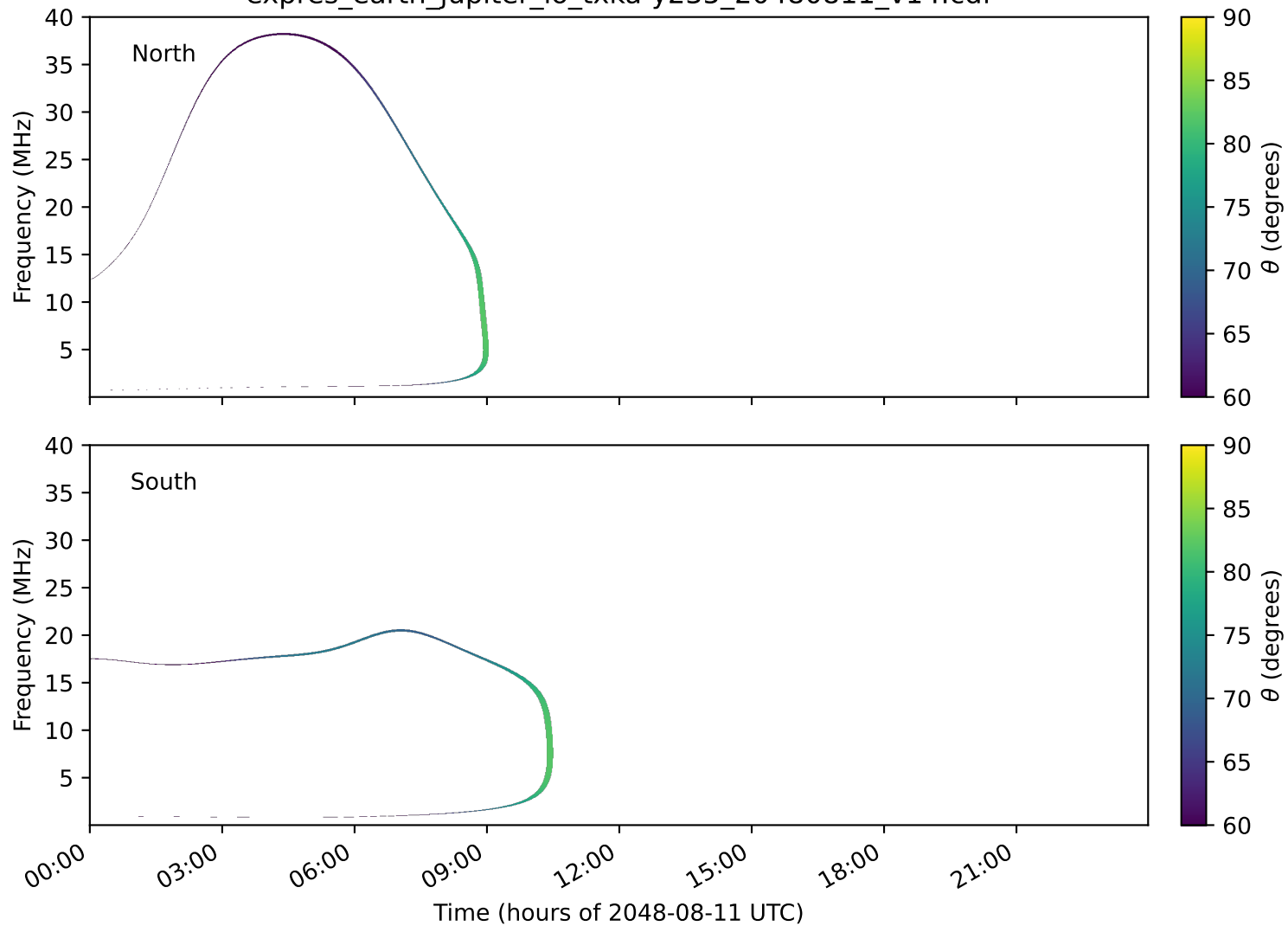
expres_earth_jupiter_io_txka-y235_20480811_v14.cdf
