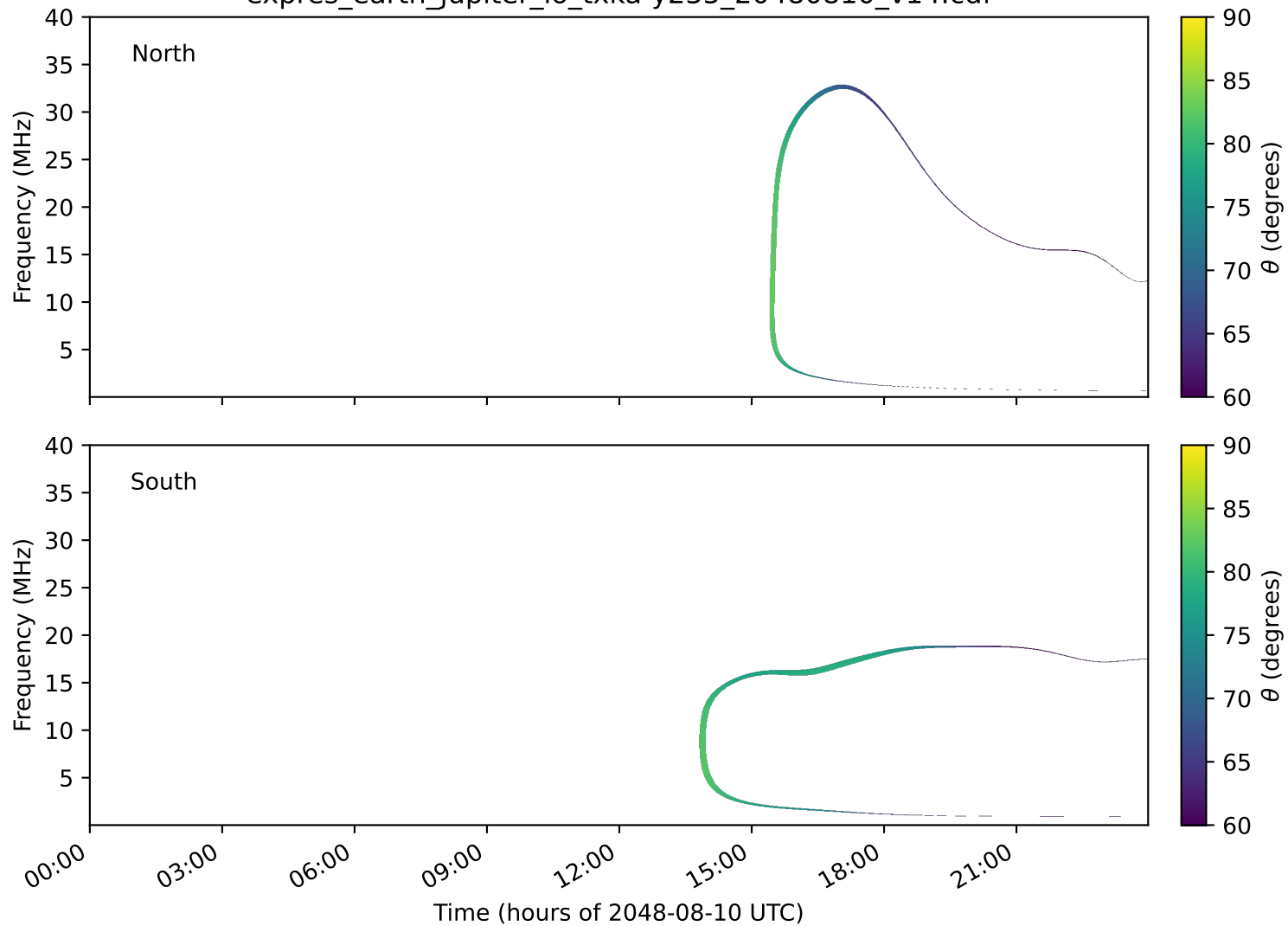
expres_earth_jupiter_io_txka-y235_20480810_v14.cdf
