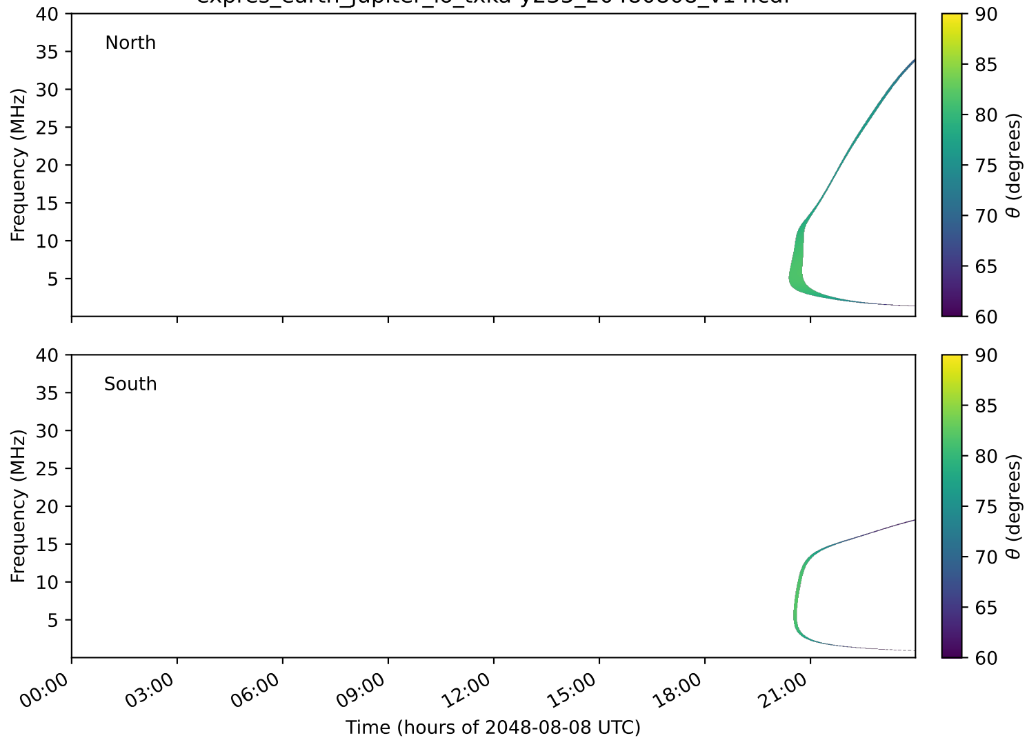
expres_earth_jupiter_io_txka-y235_20480808_v14.cdf
