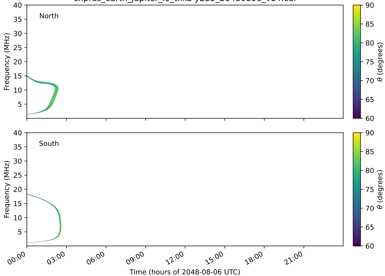
expres_earth_jupiter_io_txka-y235_20480806_v14.cdf
