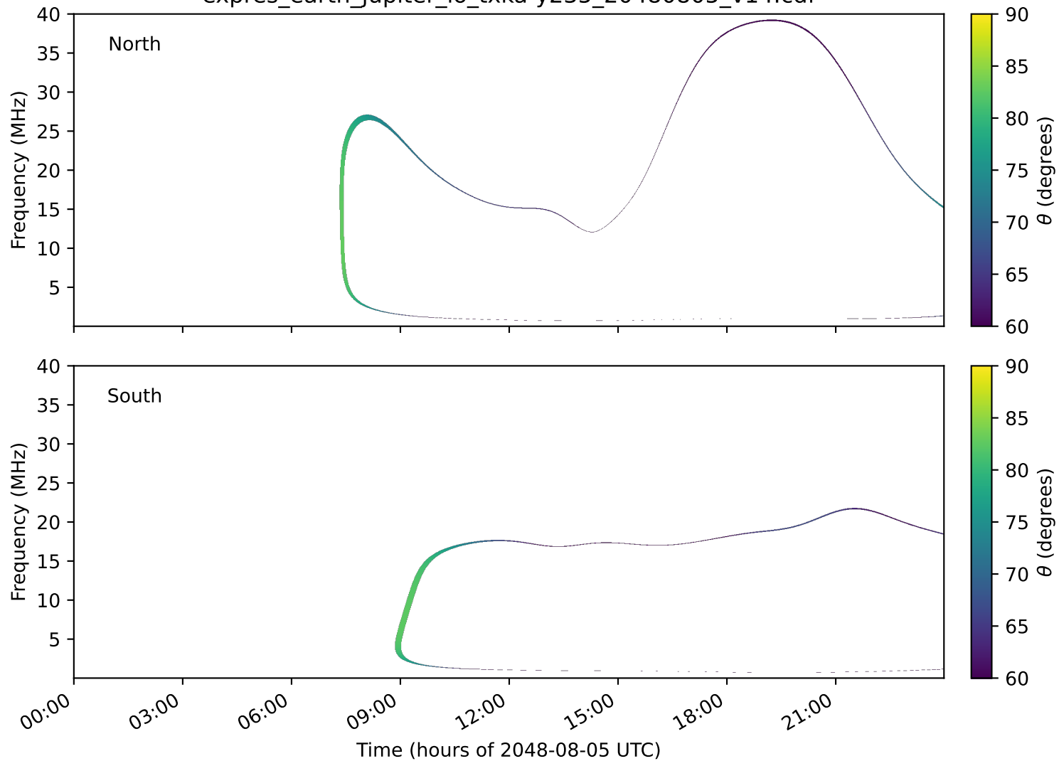
expres_earth_jupiter_io_txka-y235_20480805_v14.cdf
