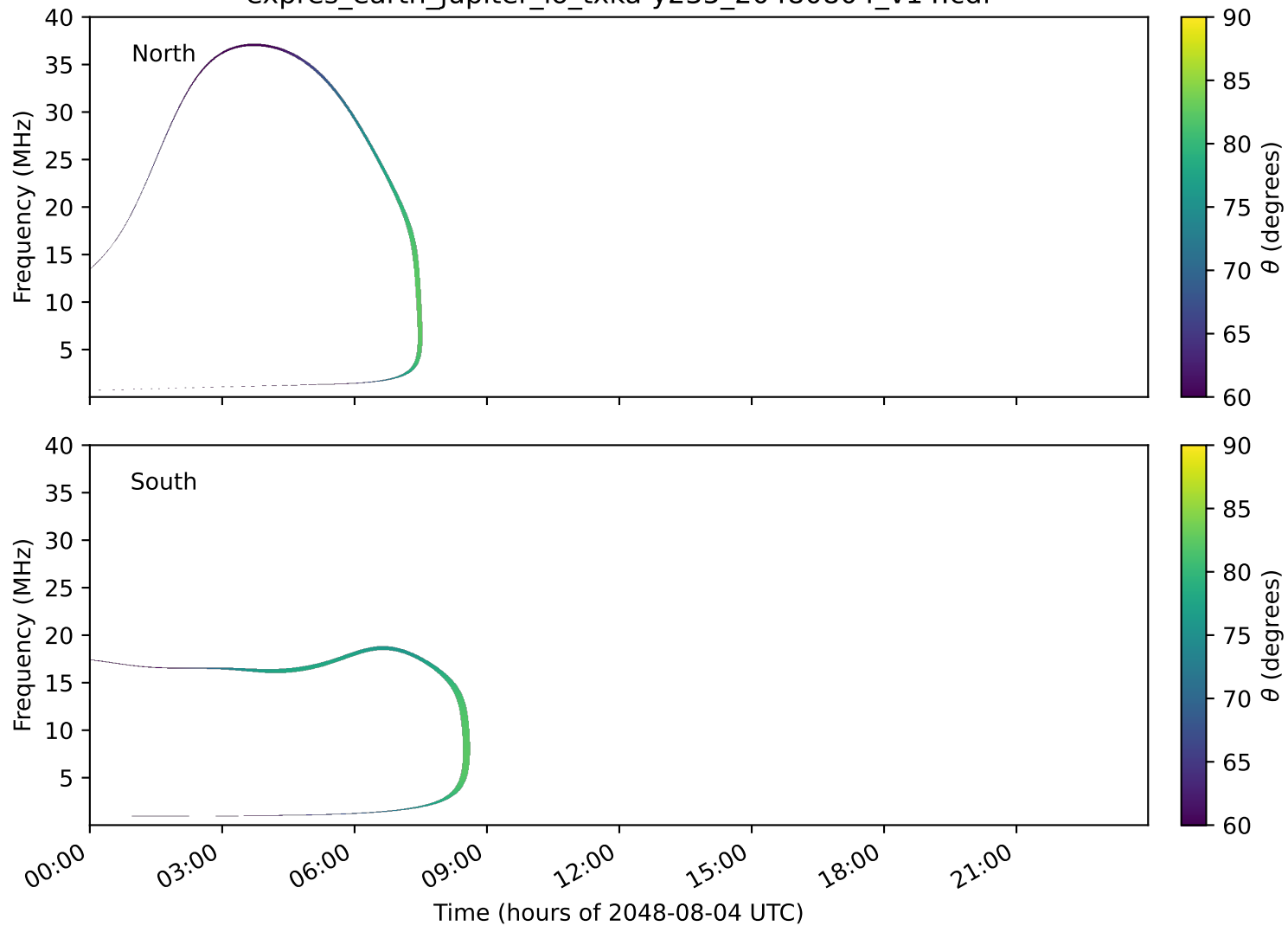
expres_earth_jupiter_io_txka-y235_20480804_v14.cdf
