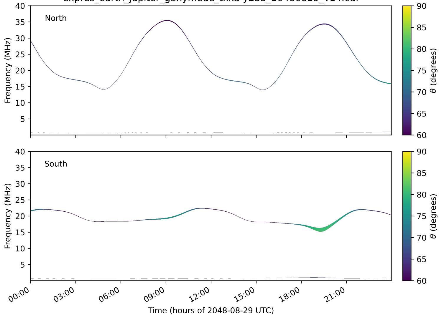
expres_earth_jupiter_ganymede_txka-y235_20480829_v14.cdf
