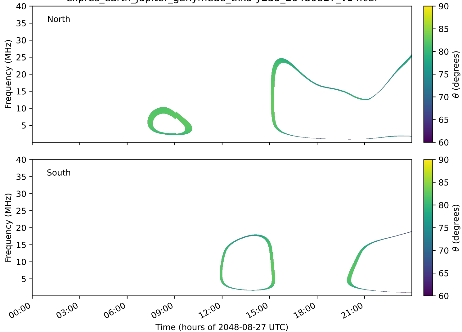
expres_earth_jupiter_ganymede_txka-y235_20480827_v14.cdf
