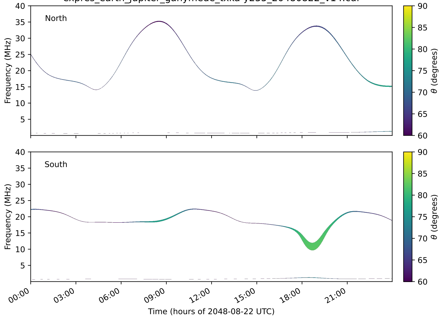
expres_earth_jupiter_ganymede_txka-y235_20480822_v14.cdf
