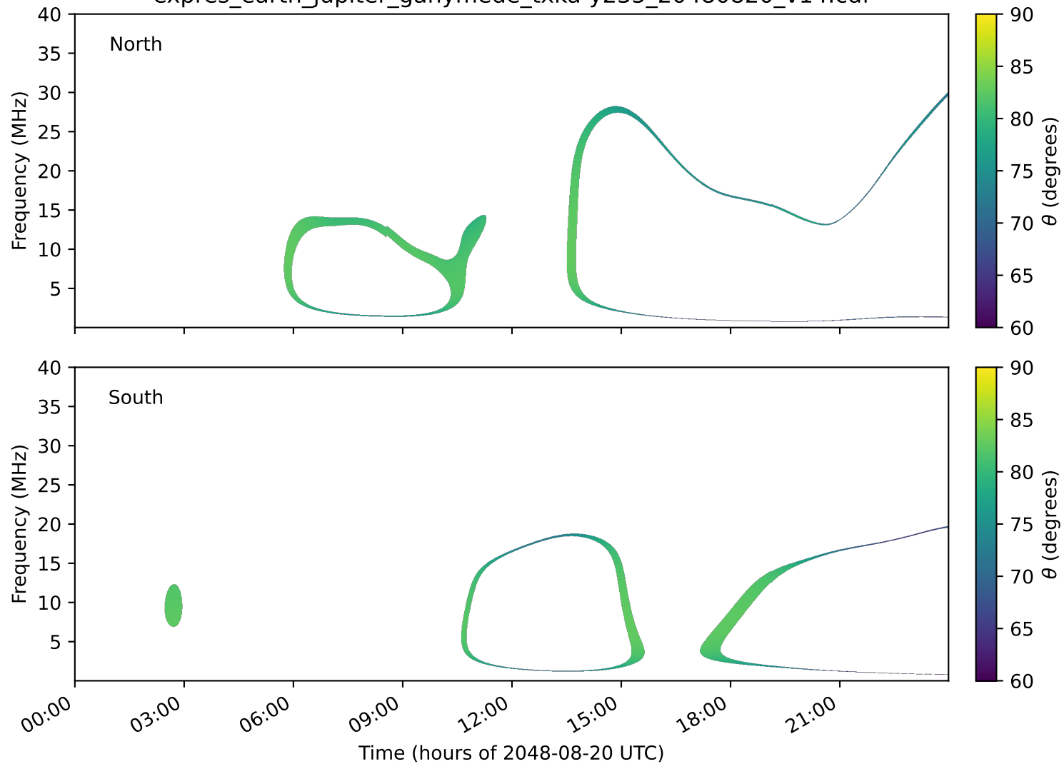
expres_earth_jupiter_ganymede_txka-y235_20480820_v14.cdf
