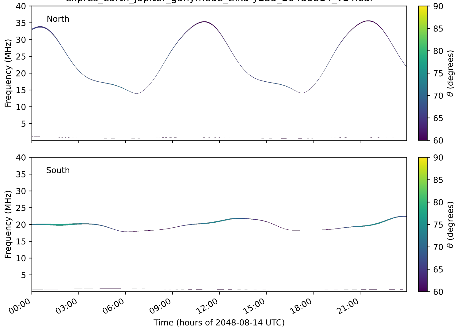
expres_earth_jupiter_ganymede_txka-y235_20480814_v14.cdf
