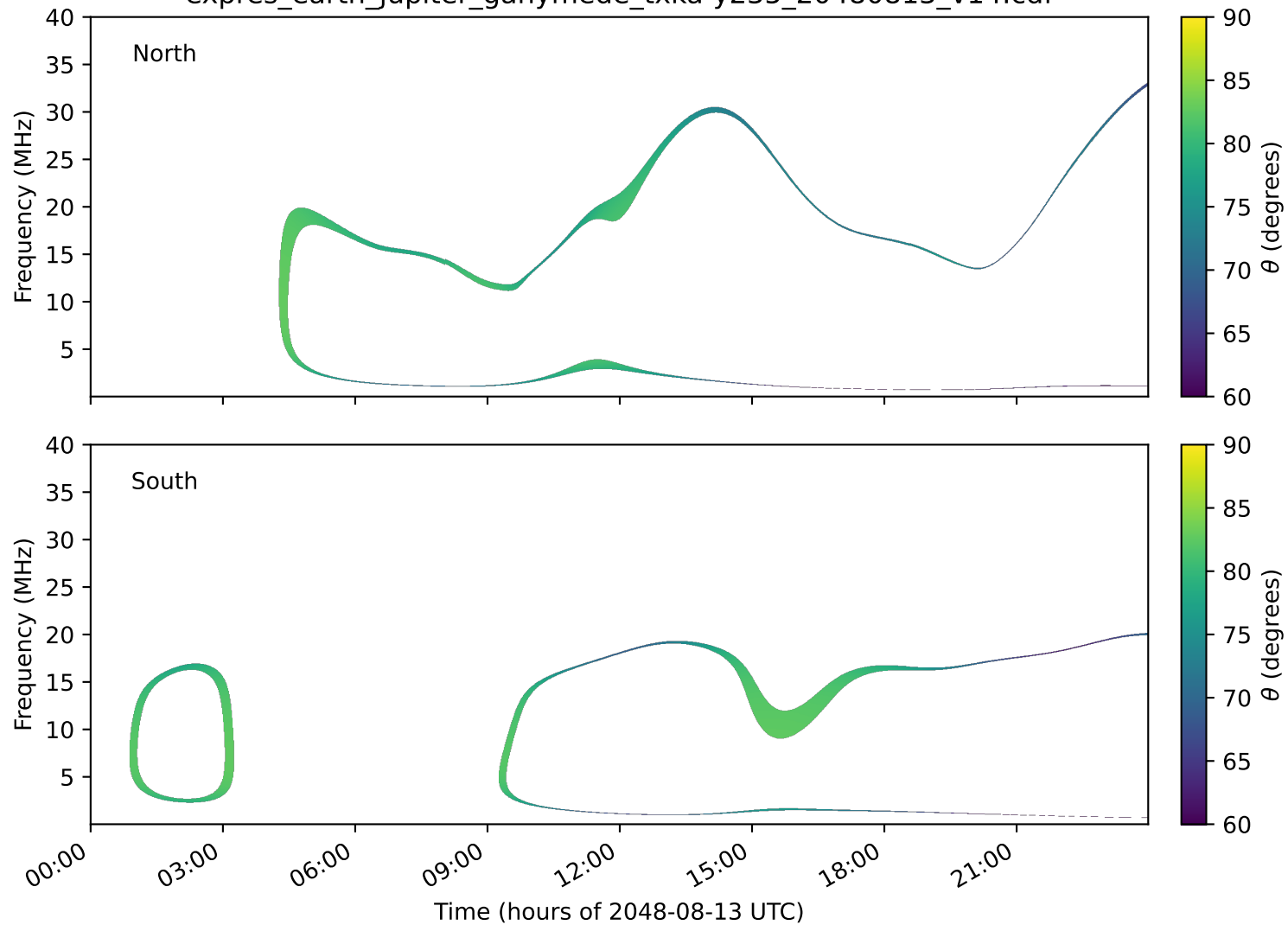
expres_earth_jupiter_ganymede_txka-y235_20480813_v14.cdf
