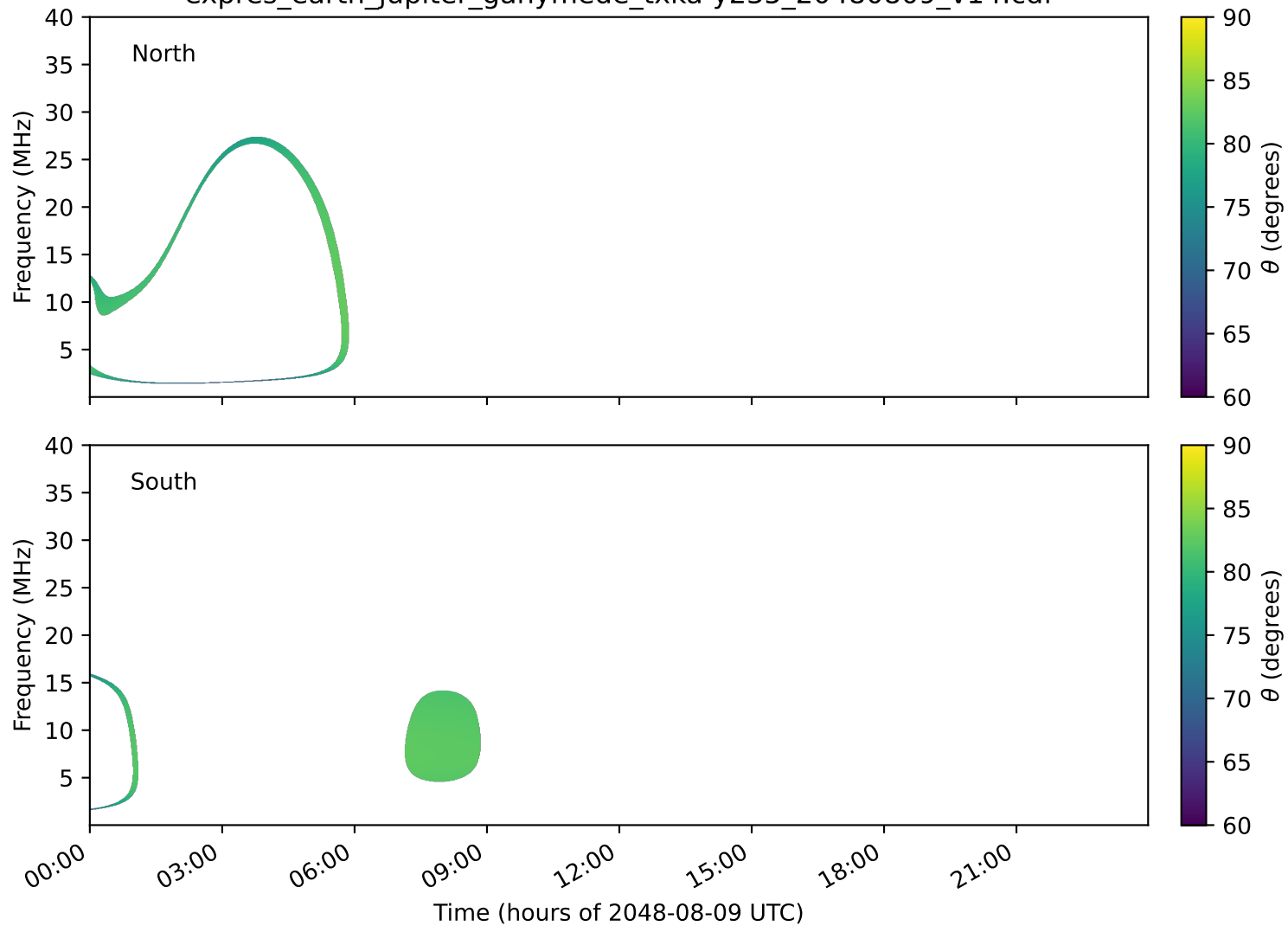
expres_earth_jupiter_ganymede_txka-y235_20480809_v14.cdf
