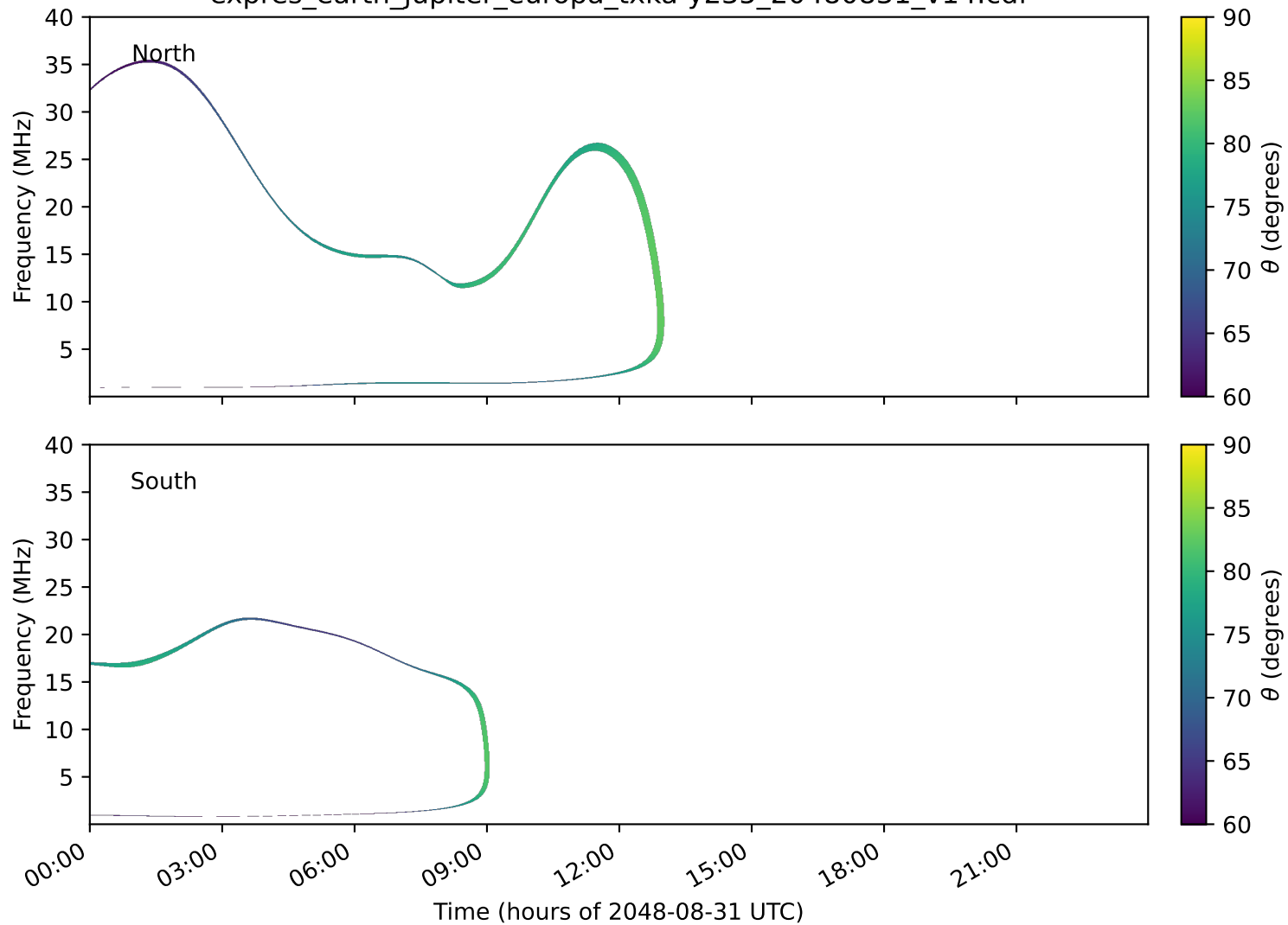
expres_earth_jupiter_europa_txka-y235_20480831_v14.cdf
