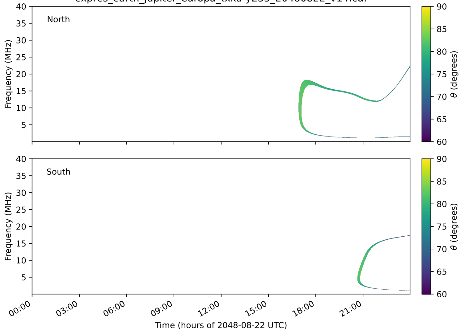
expres_earth_jupiter_europa_txka-y235_20480822_v14.cdf
