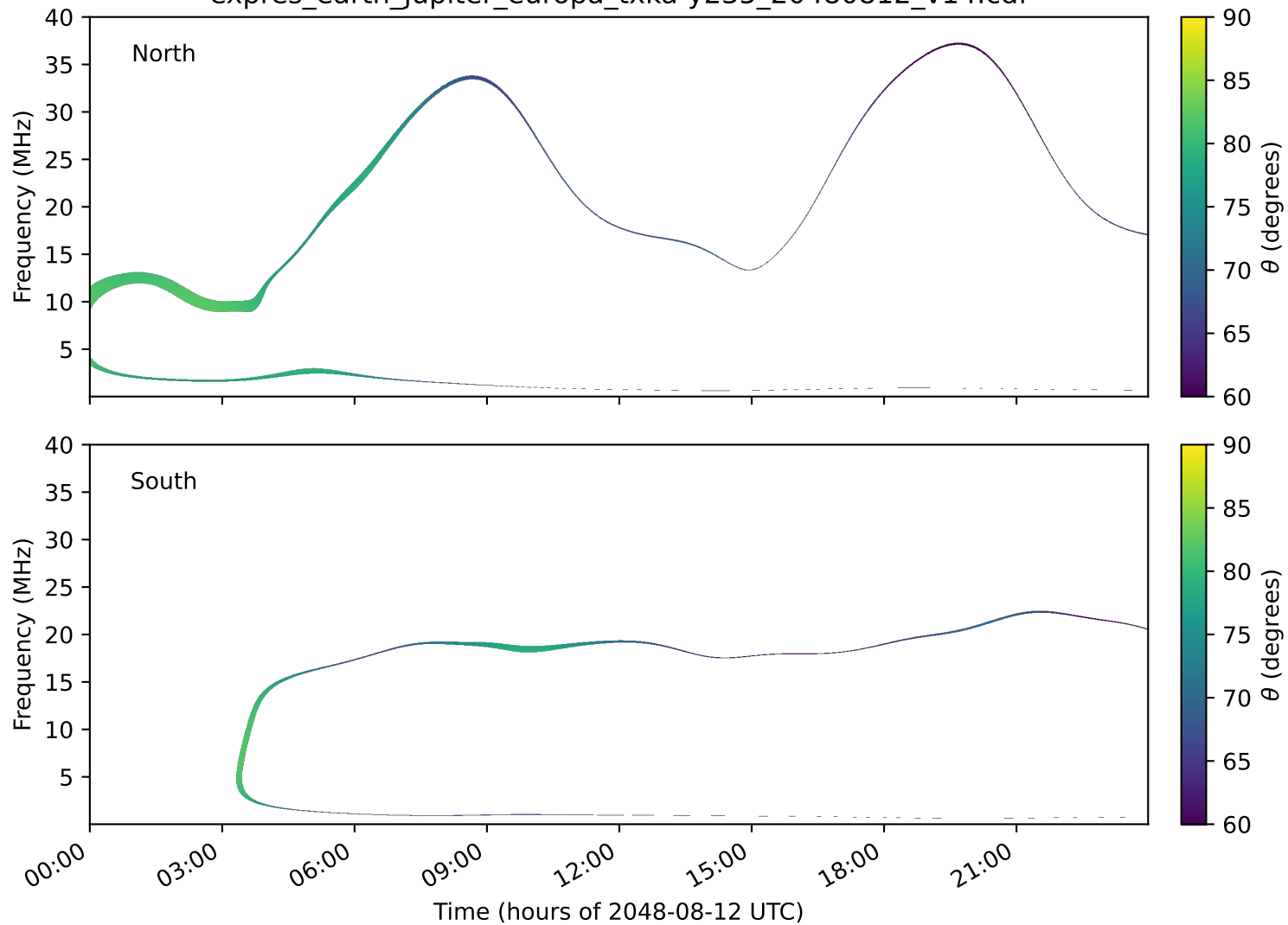
expres_earth_jupiter_europa_txka-y235_20480812_v14.cdf
