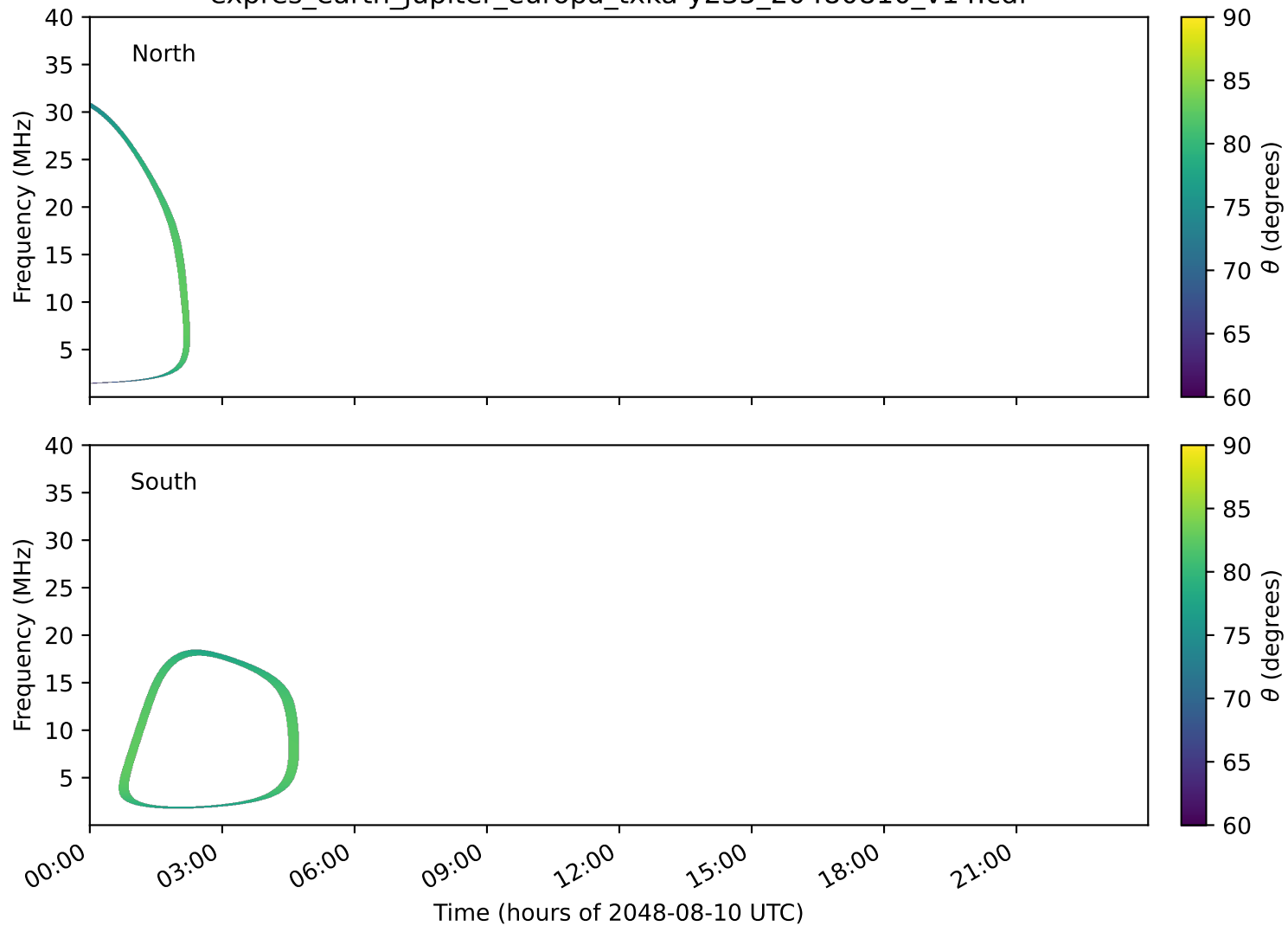
expres_earth_jupiter_europa_txka-y235_20480810_v14.cdf
