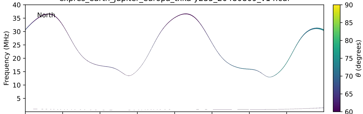
expres_earth_jupiter_europa_txka-y235_20480809_v14.cdf
