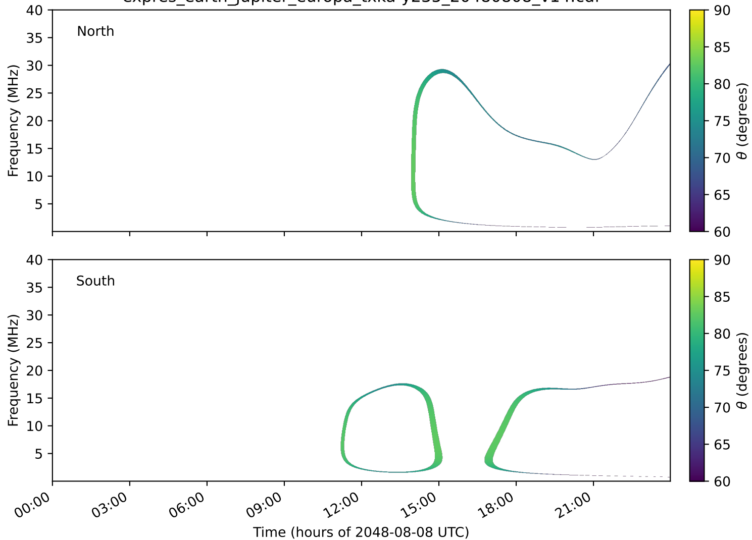
expres_earth_jupiter_europa_txka-y235_20480808_v14.cdf
