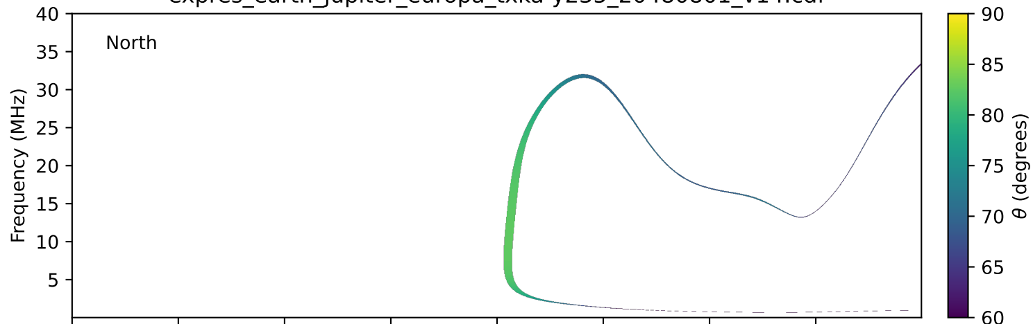
expres_earth_jupiter_europa_txka-y235_20480801_v14.cdf
