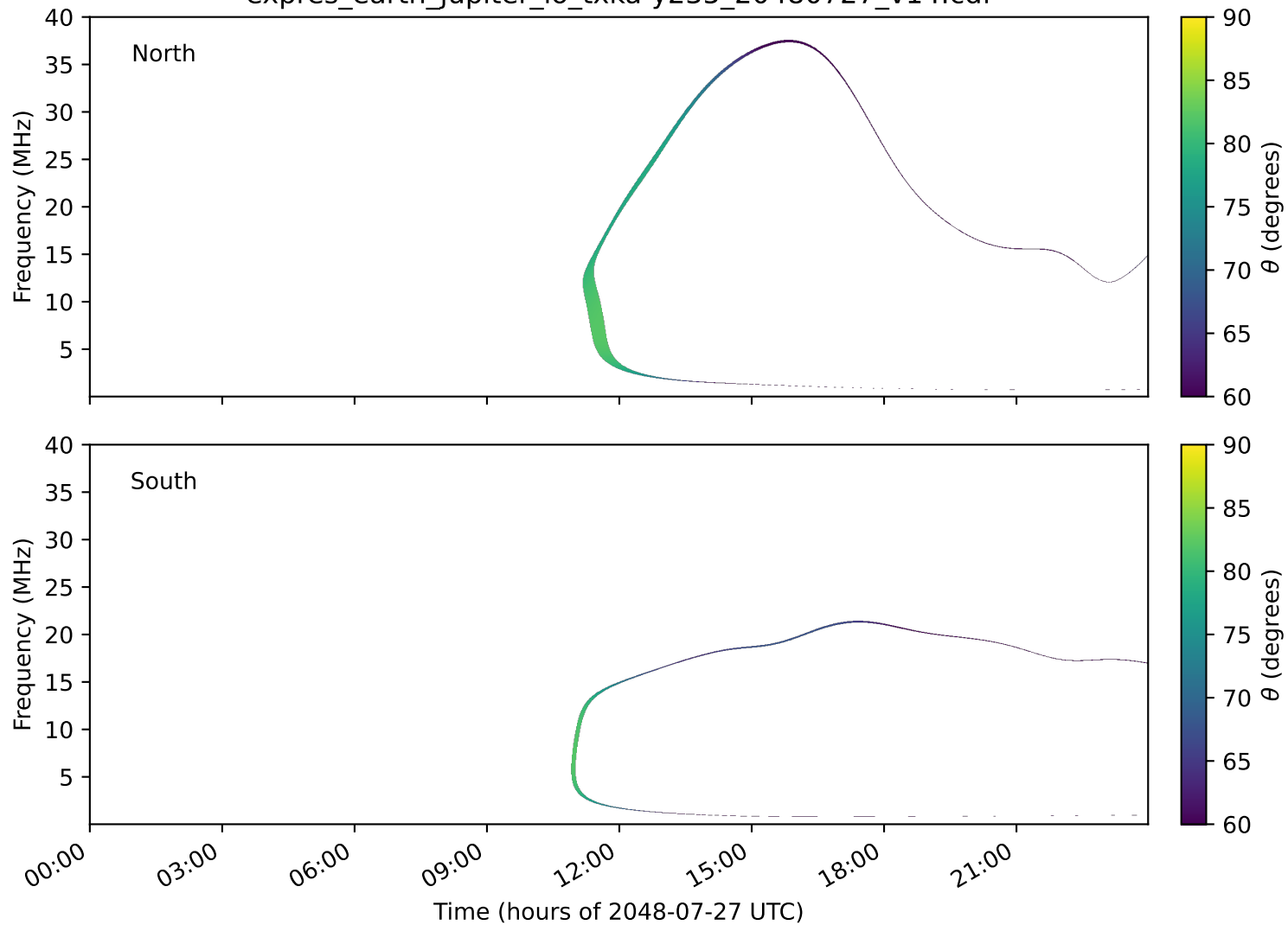
expres_earth_jupiter_io_txka-y235_20480727_v14.cdf
