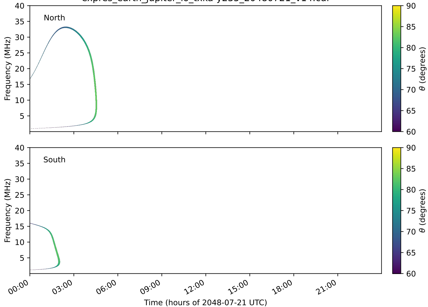
expres_earth_jupiter_io_txka-y235_20480721_v14.cdf
