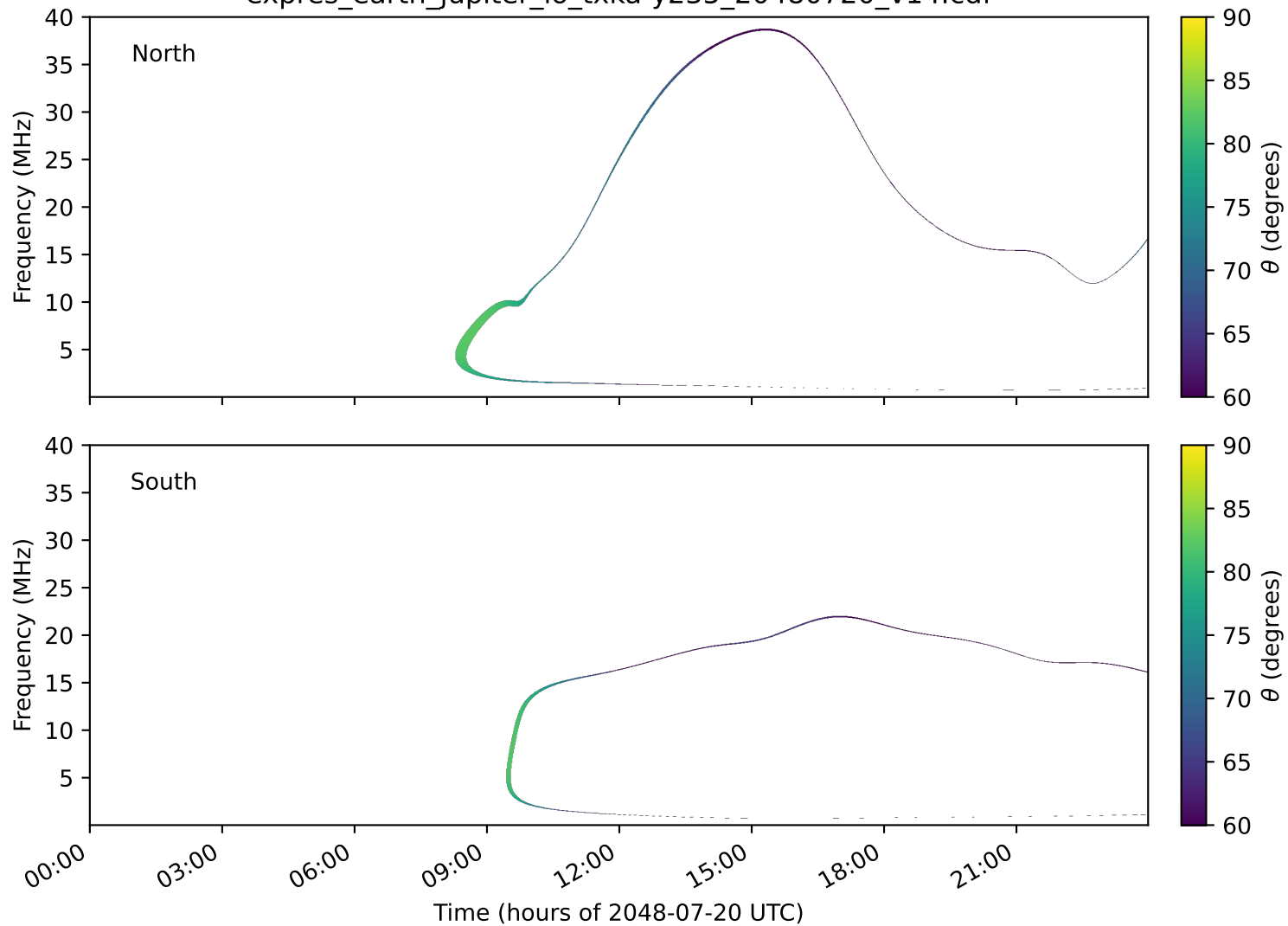
expres_earth_jupiter_io_txka-y235_20480720_v14.cdf
