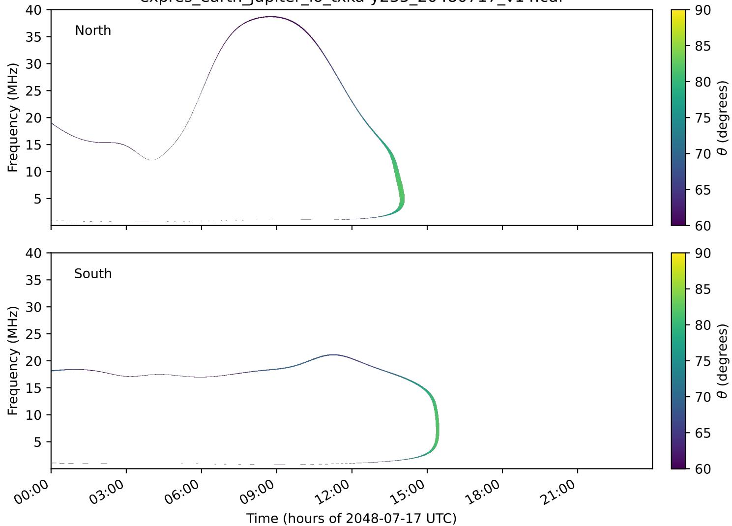
expres_earth_jupiter_io_txka-y235_20480717_v14.cdf
