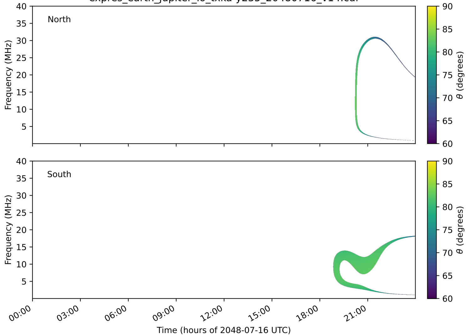
expres_earth_jupiter_io_txka-y235_20480716_v14.cdf
