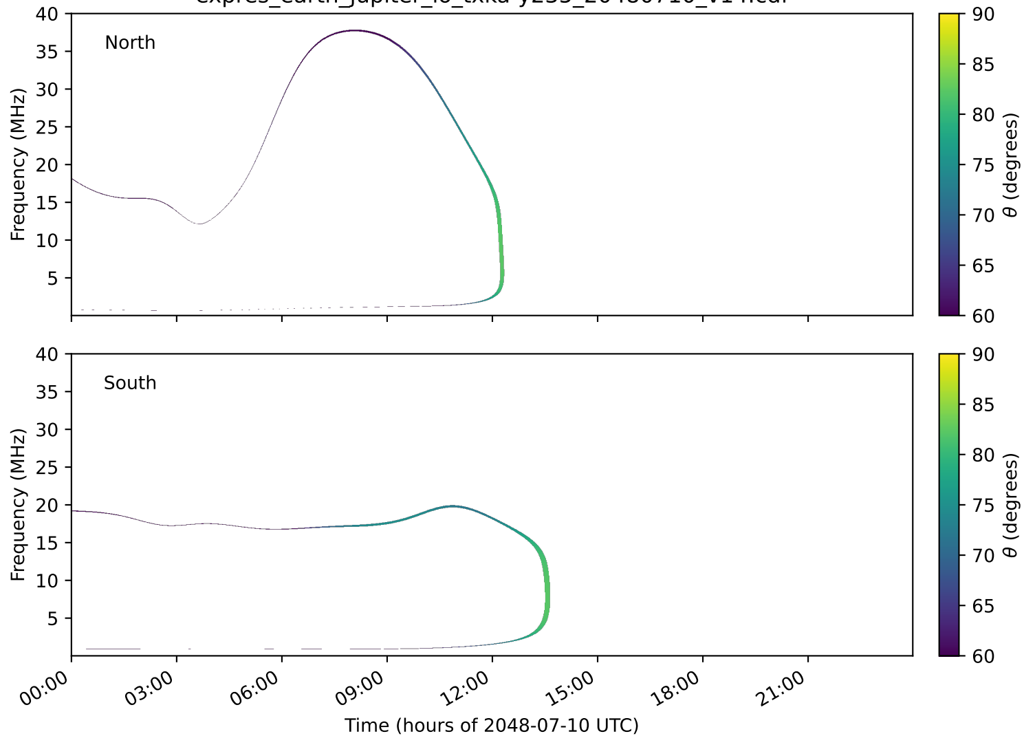
expres_earth_jupiter_io_txka-y235_20480710_v14.cdf
