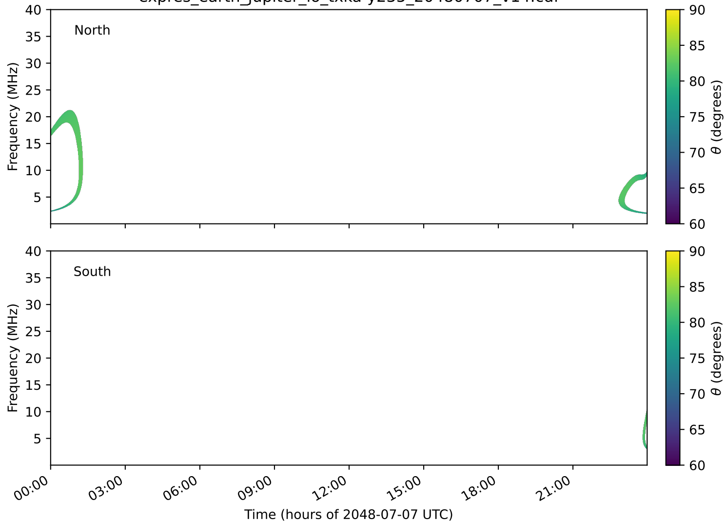
expres_earth_jupiter_io_txka-y235_20480707_v14.cdf
