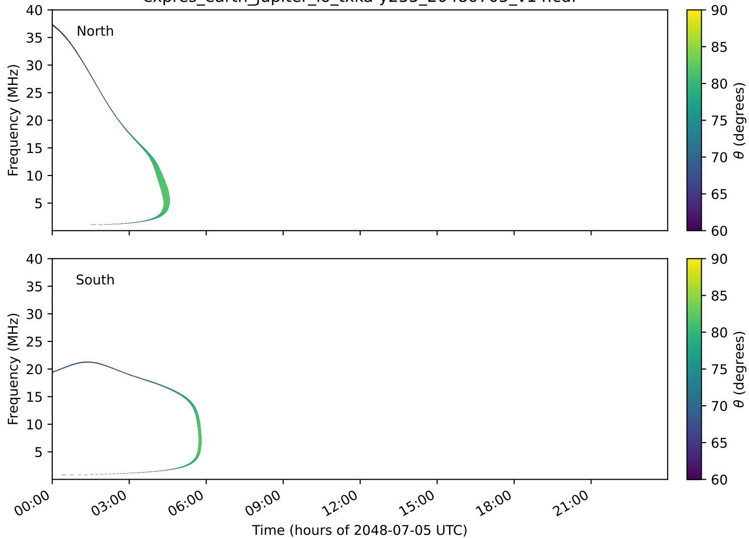
expres_earth_jupiter_io_txka-y235_20480705_v14.cdf
