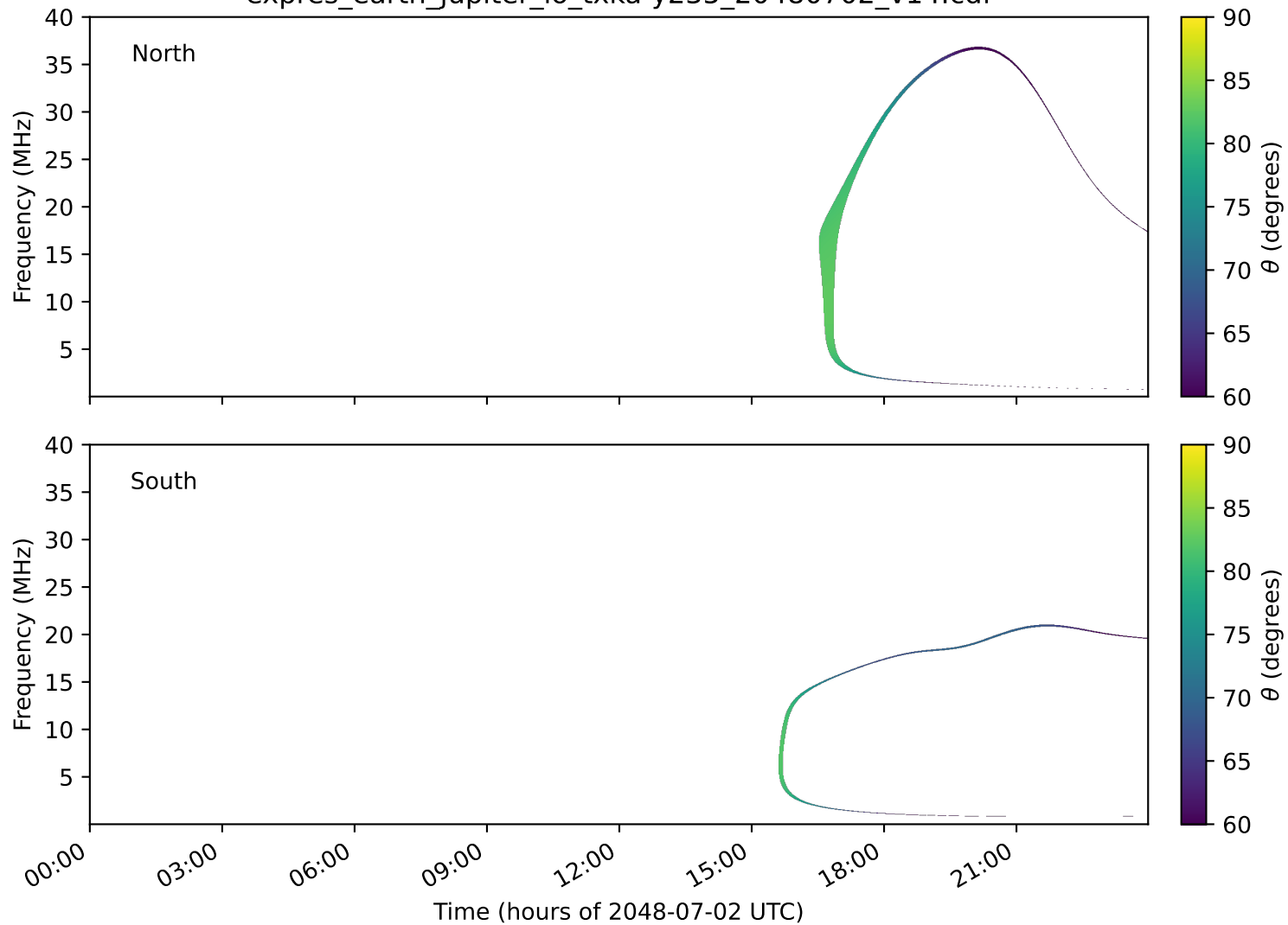
expres_earth_jupiter_io_txka-y235_20480702_v14.cdf
