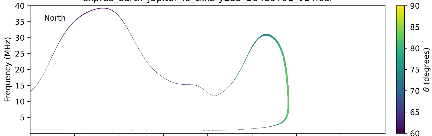
expres_earth_jupiter_io_txka-y235_20480701_v14.cdf
