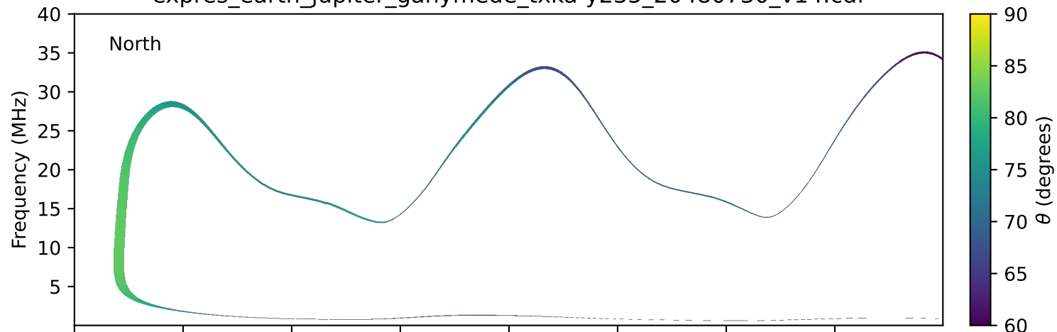
expres_earth_jupiter_ganymede_txka-y235_20480730_v14.cdf
