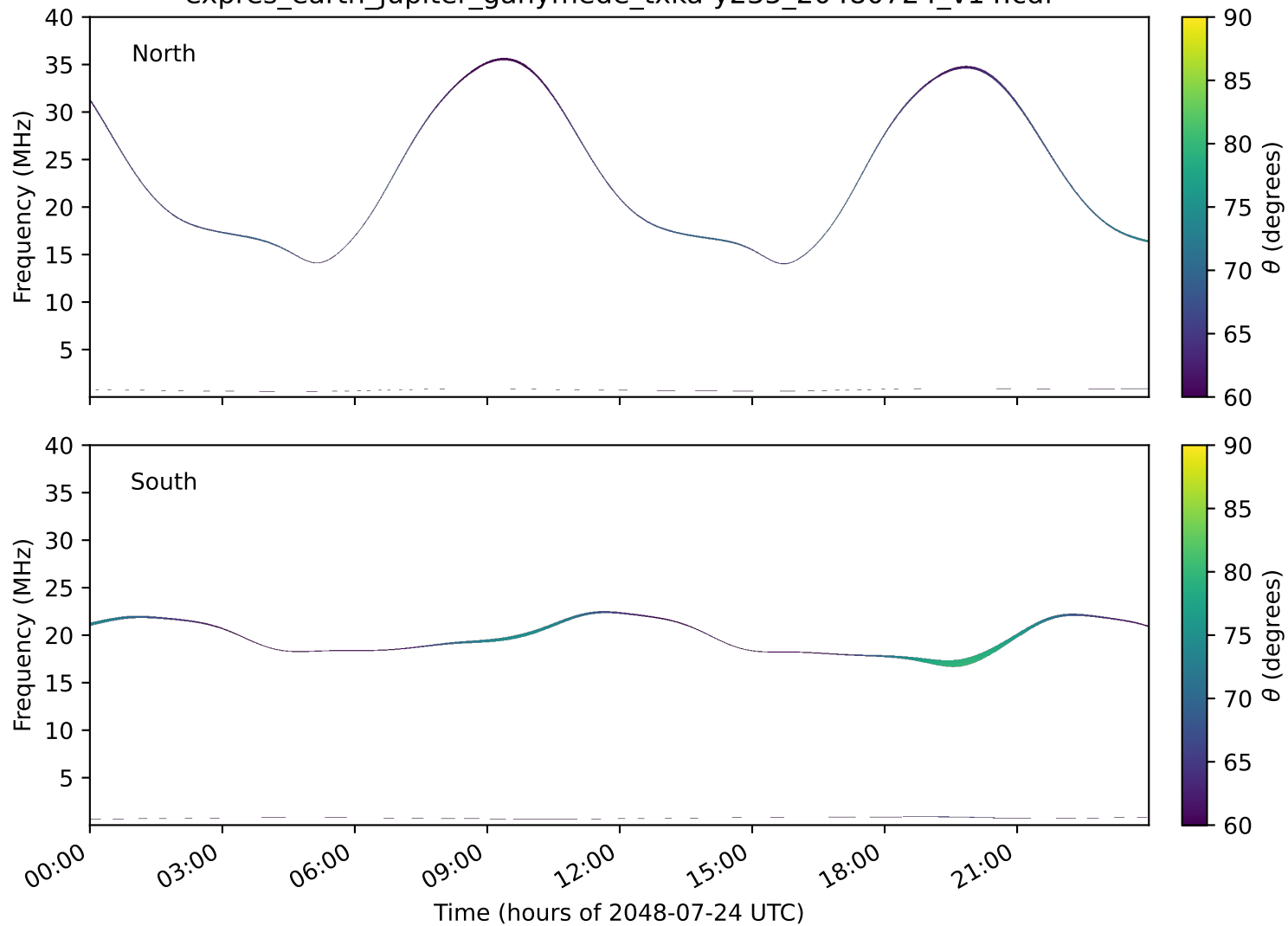
expres_earth_jupiter_ganymede_txka-y235_20480724_v14.cdf
