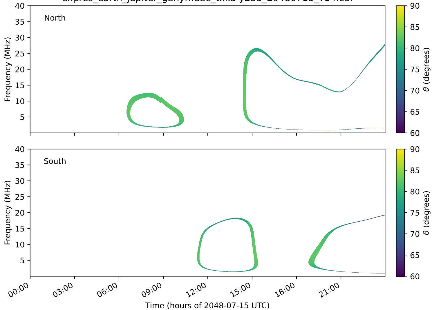
expres_earth_jupiter_ganymede_txka-y235_20480715_v14.cdf
