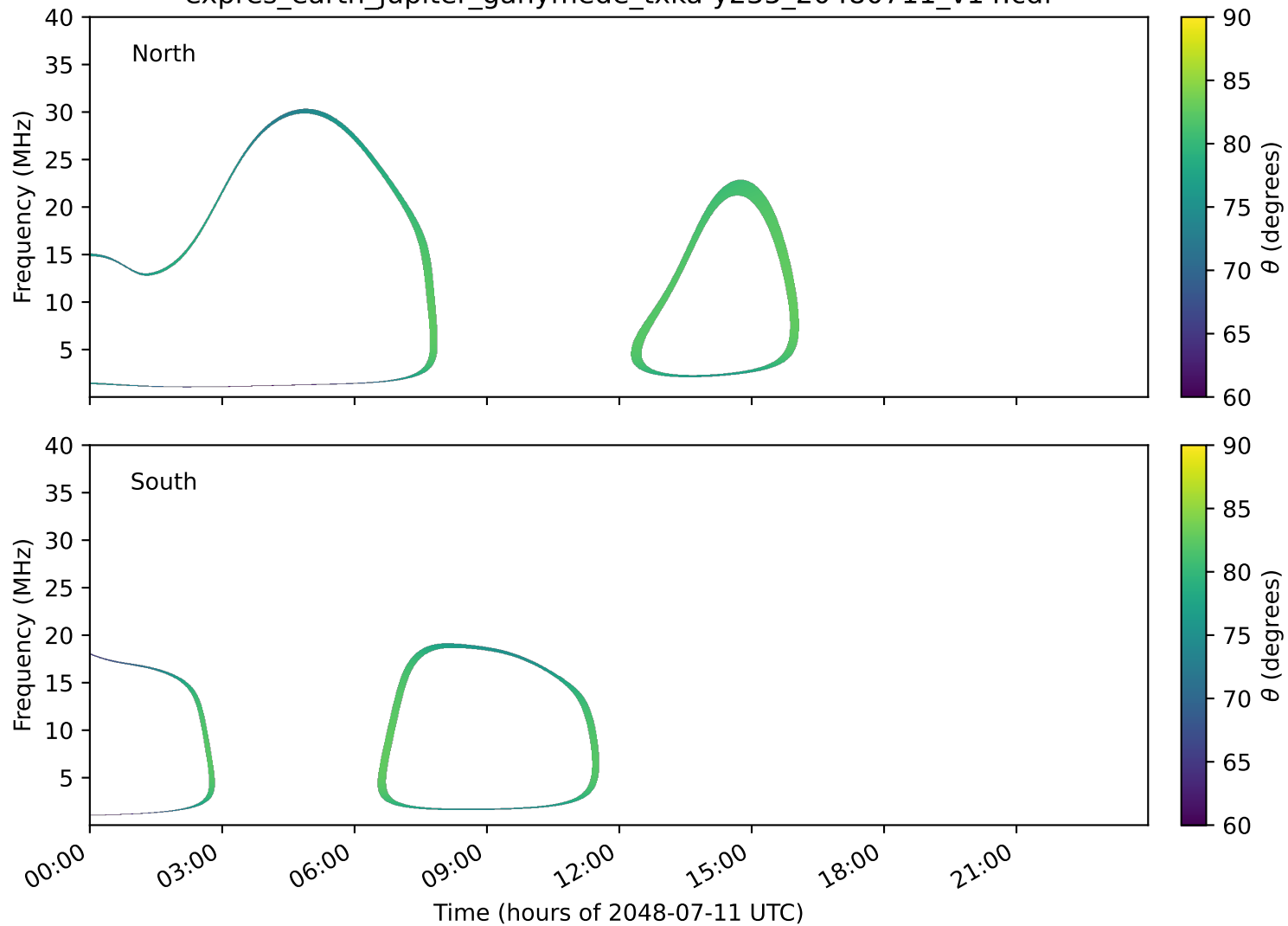
expres_earth_jupiter_ganymede_txka-y235_20480711_v14.cdf
