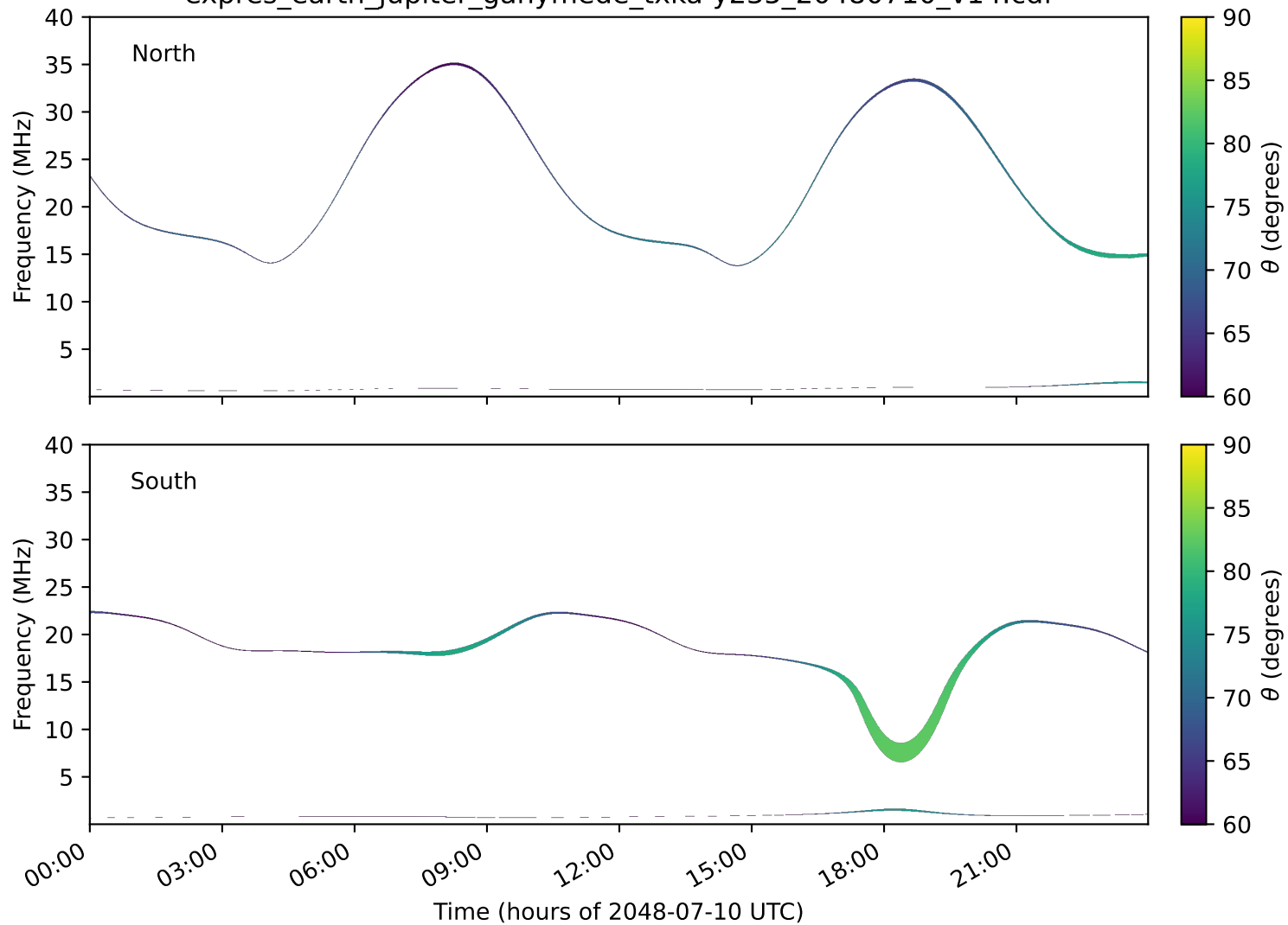
expres_earth_jupiter_ganymede_txka-y235_20480710_v14.cdf
