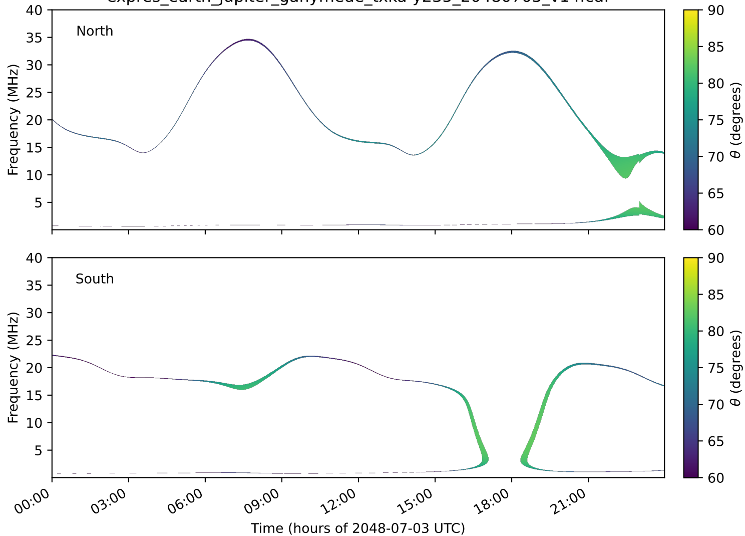
expres_earth_jupiter_ganymede_txka-y235_20480703_v14.cdf
