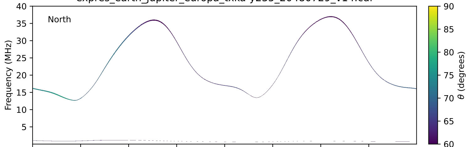
expres_earth_jupiter_europa_txka-y235_20480729_v14.cdf
