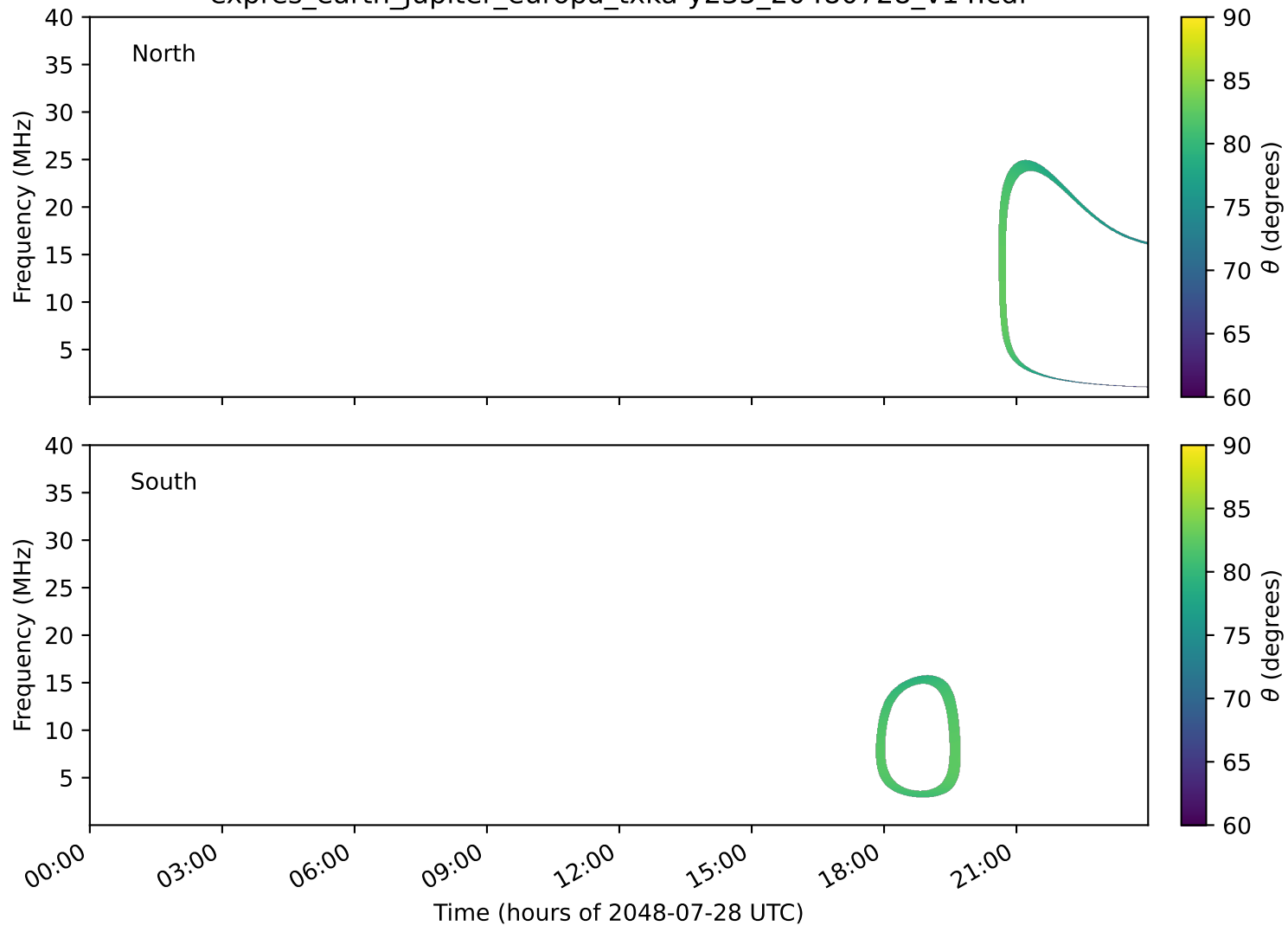
expres_earth_jupiter_europa_txka-y235_20480728_v14.cdf
