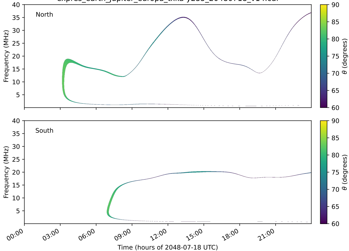
expres_earth_jupiter_europa_txka-y235_20480718_v14.cdf
