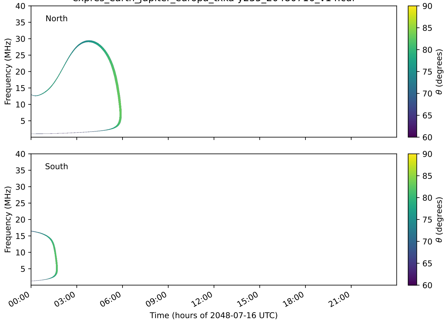
expres_earth_jupiter_europa_txka-y235_20480716_v14.cdf
