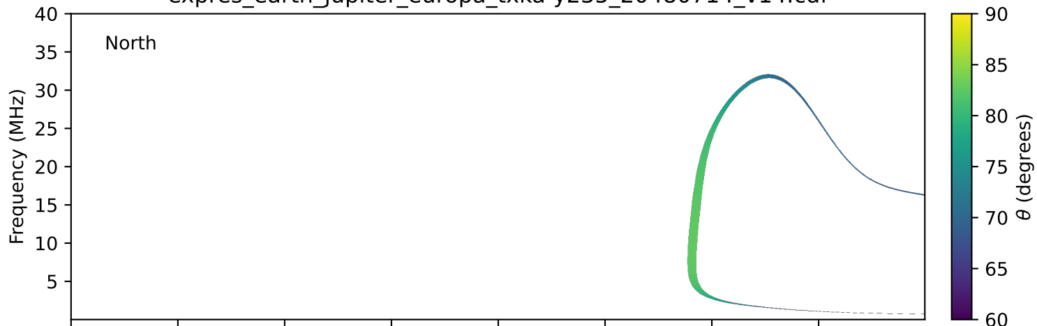
expres_earth_jupiter_europa_txka-y235_20480714_v14.cdf
