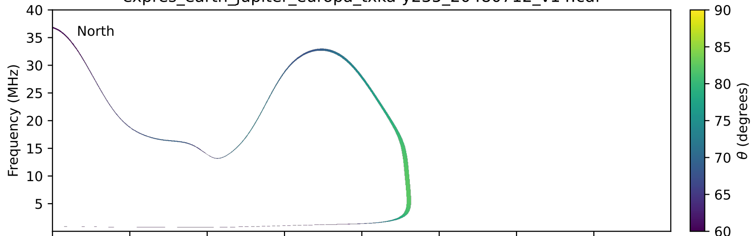
expres_earth_jupiter_europa_txka-y235_20480712_v14.cdf
