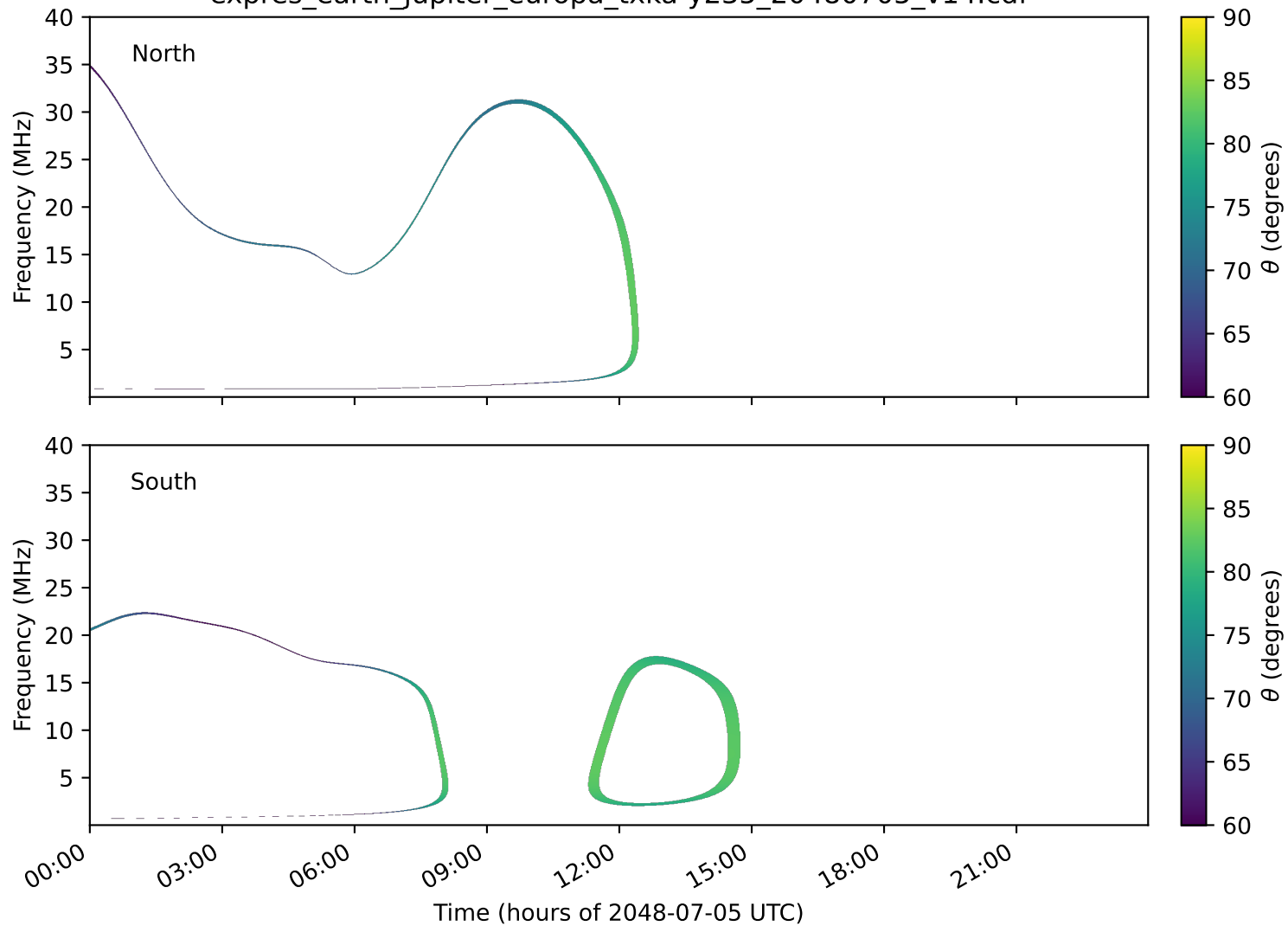
expres_earth_jupiter_europa_txka-y235_20480705_v14.cdf
